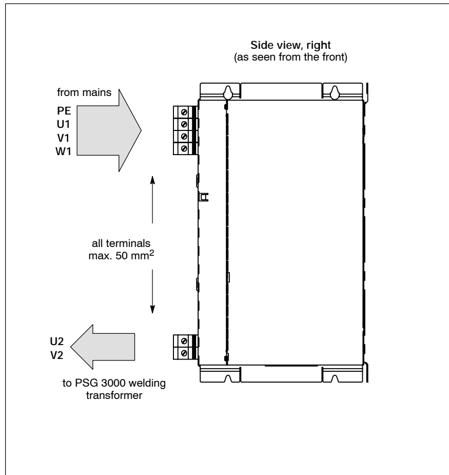
Electrical connection, PSI 6100.XXX L1/L2/W1/W2
