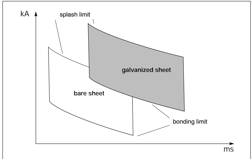
Welding of different sheet types, conventional 50/60 Hz weld
