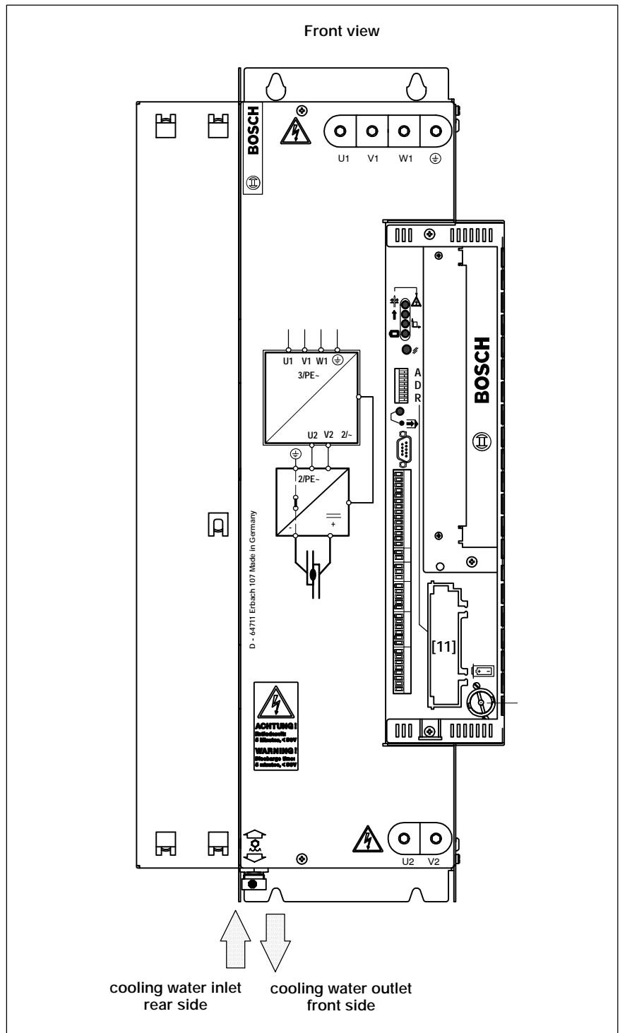
Cooling water connection, PSI 6200.XXX W1/W2
