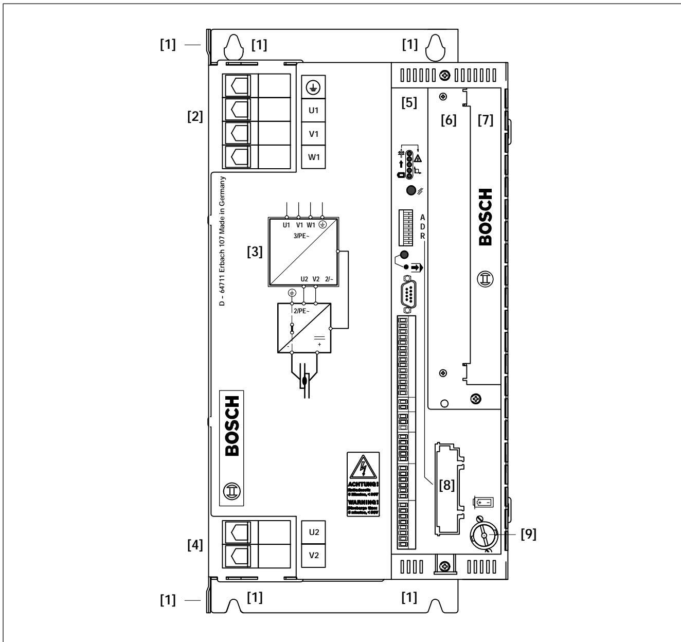
PSI 6025.XXX L1 front panel
