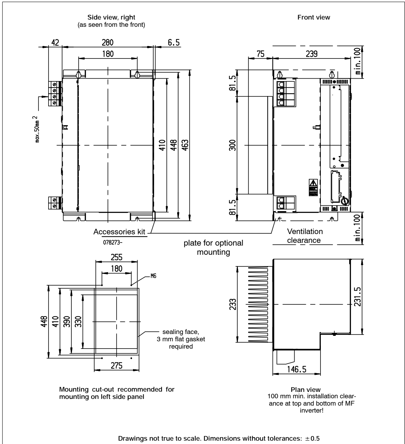
Dimensioned drawing, PSI 6100.XXX L1/L2
