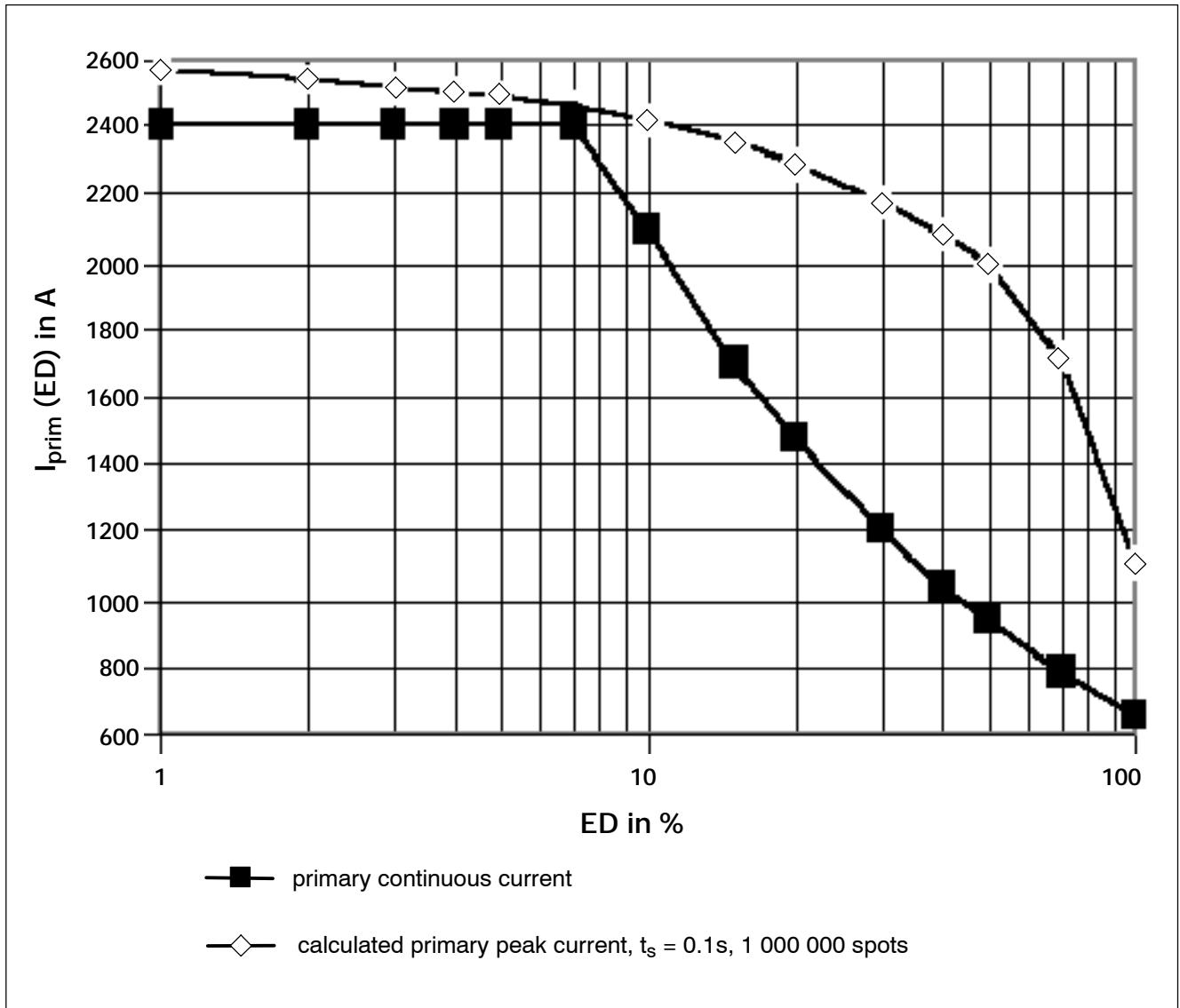
Load diagram, PSI 6500.XXX W1
