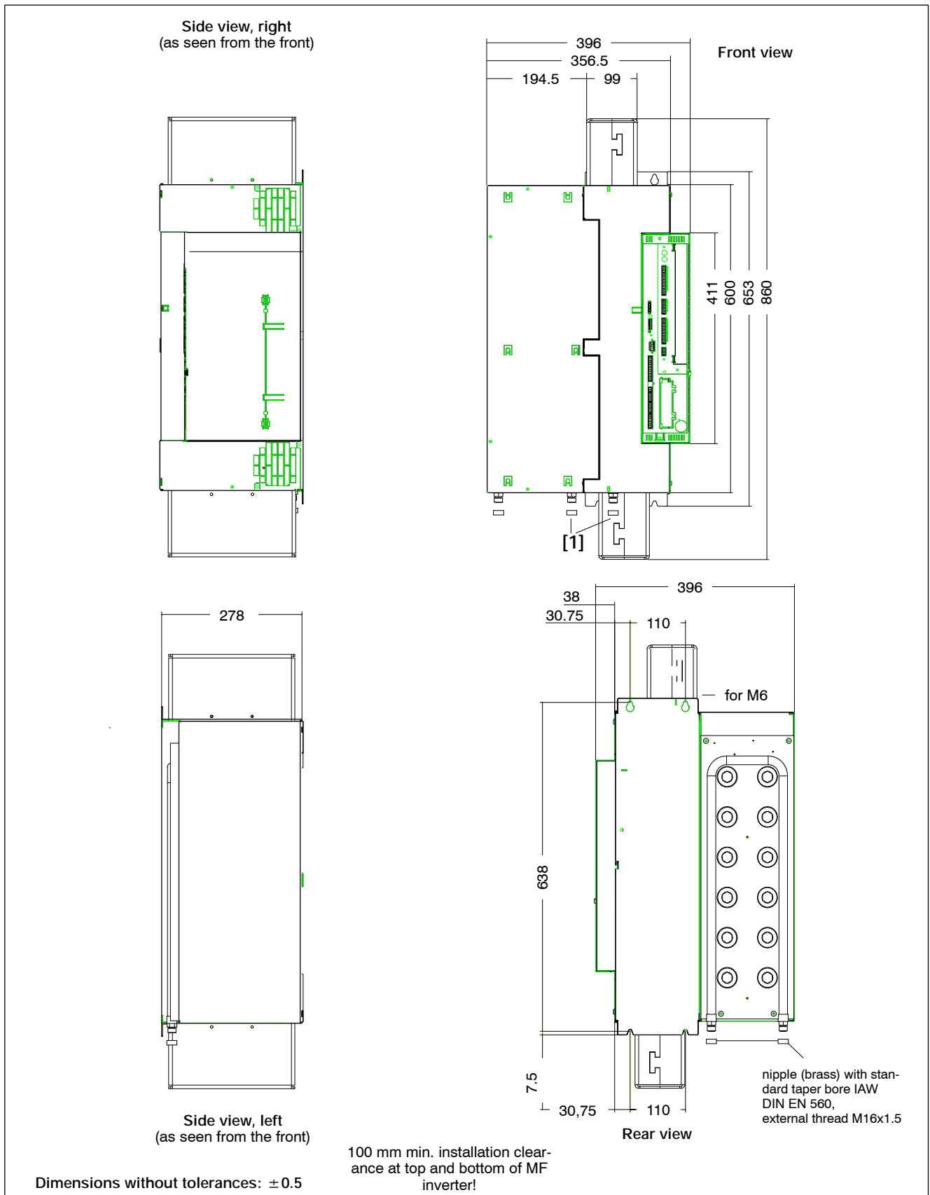
Dimensioned drawing, PSI 6500.XXX W1
