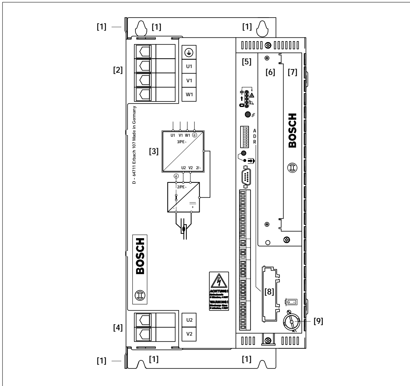
PSI 6300.XXX L1/L2/W1/W2 front panel
