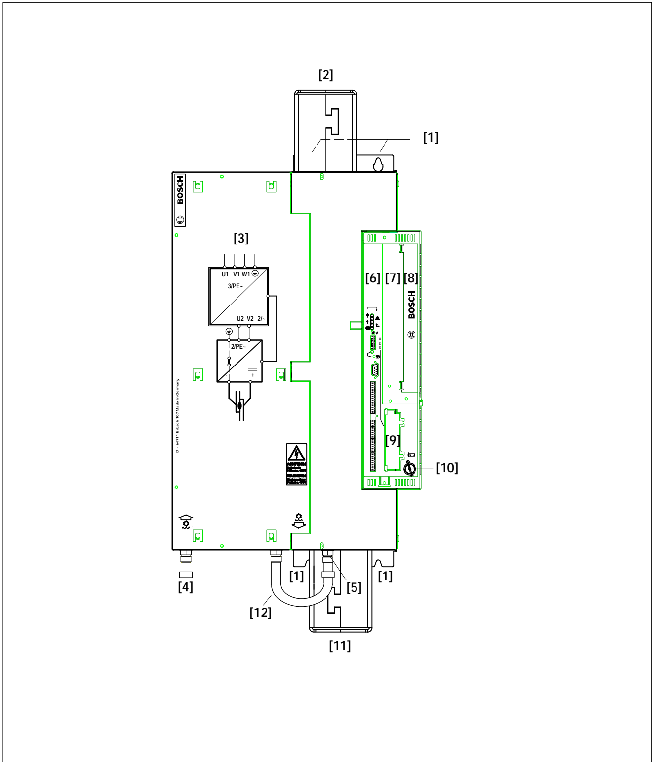
PSI 6500.XXX W1 front panel
