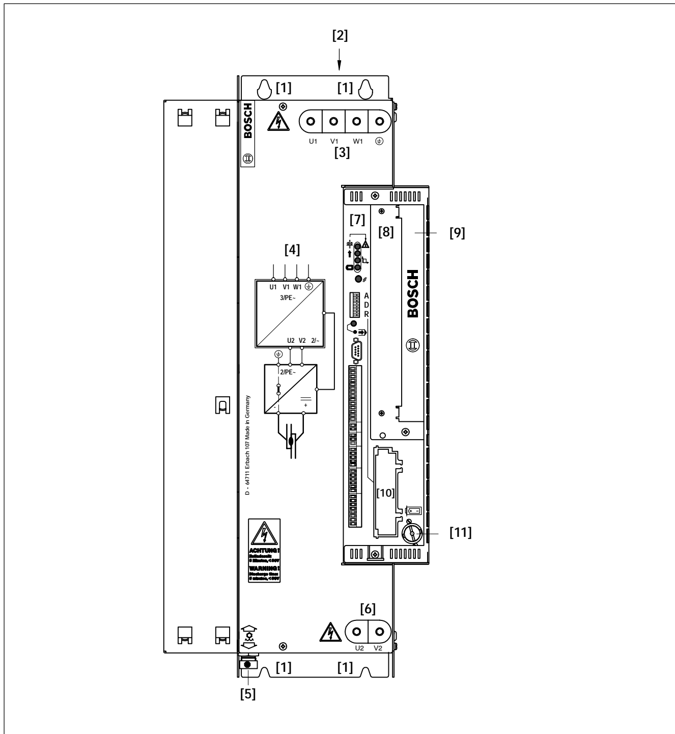
PSI 6200.XXX W1/W2 front panel
