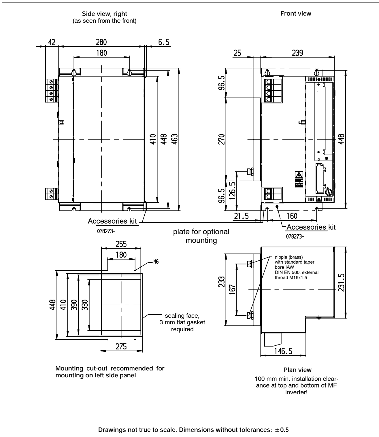
Dimensioned drawing, PSI 6300.XXX W1/W2
