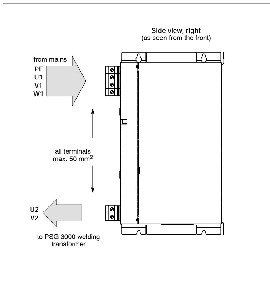
Electrical connection, PSI 6300.XXX L1/L2/W1/W2
