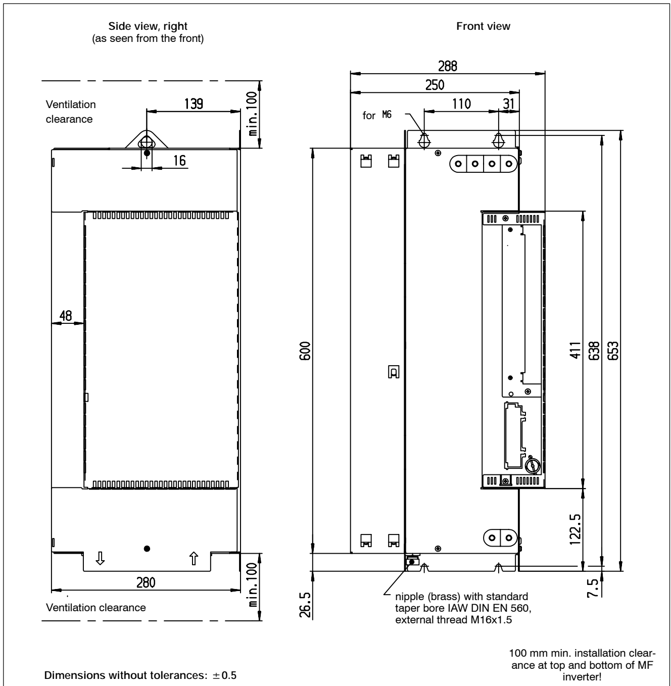
Dimensioned drawing, PSI 6200.XXX W1/W2
