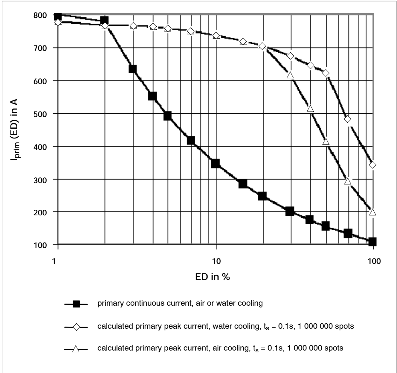
Load diagram, PSI 6300.XXX L1/W1
