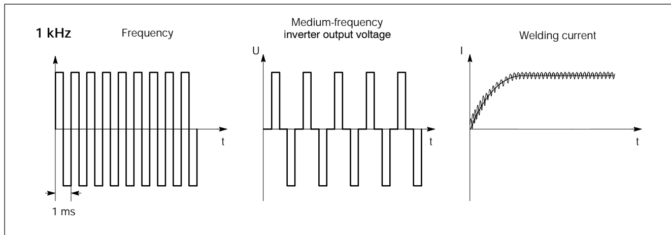
Medium-frequency welding
