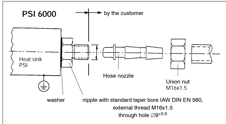
Cooling water connection
