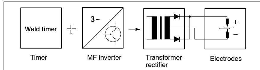
Basic functional design of the 1 kHz MF welding process
