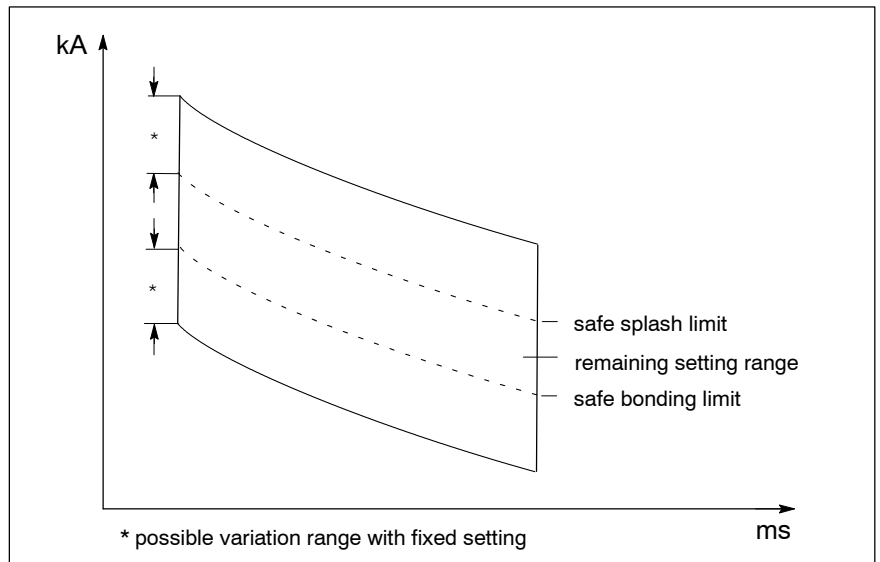
Welding of galvanized sheet types with 1 kHz welding process
