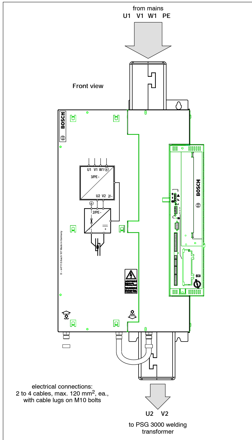
Electrical connection, PSI 6500.XXX W1
