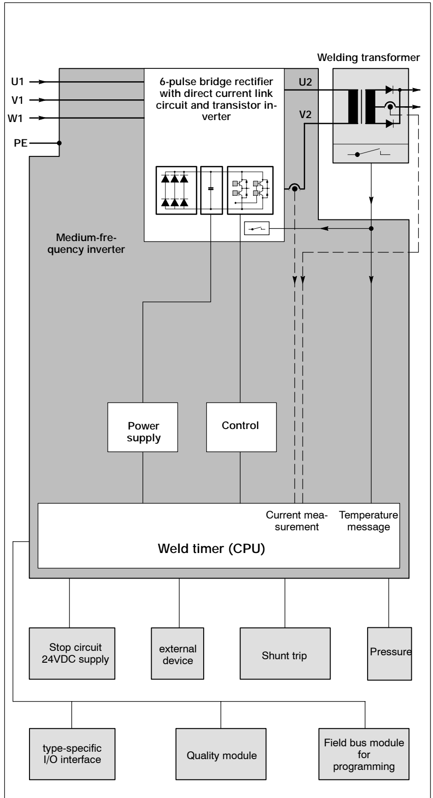
Block diagram of a medium-frequency inverter
