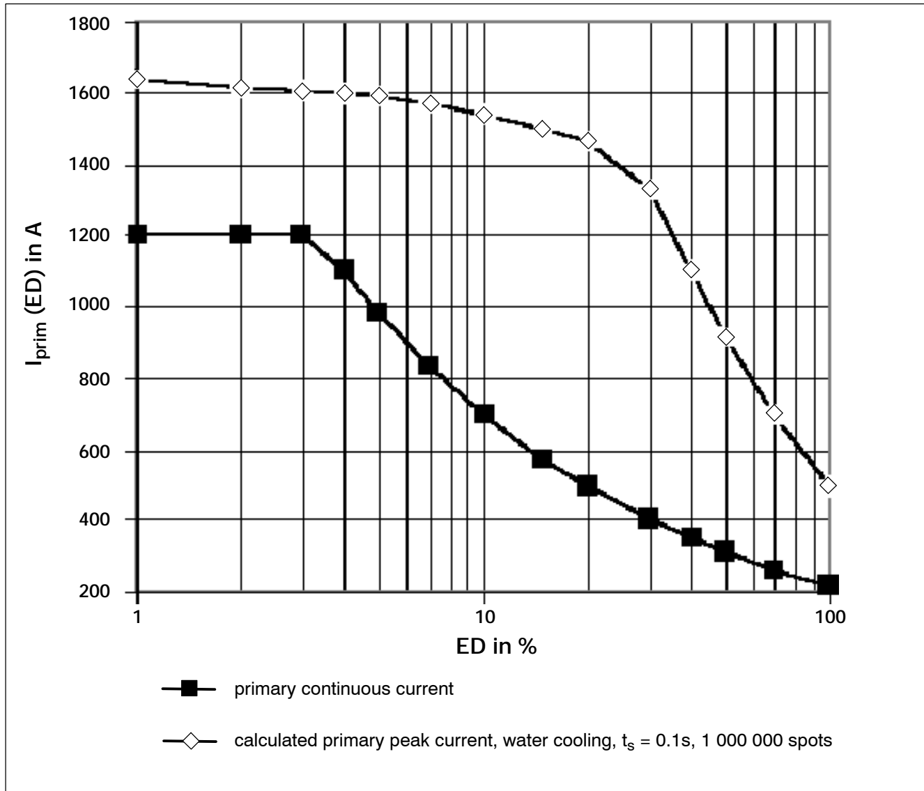
Load diagram, PSI 6200.XXX W2
