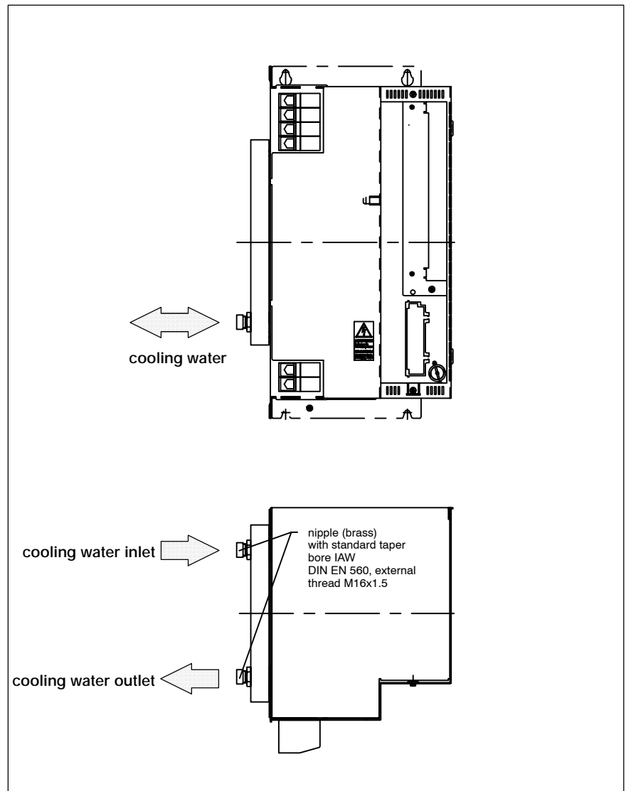
Cooling water connection, PSI 6100.XXX W1/W2
