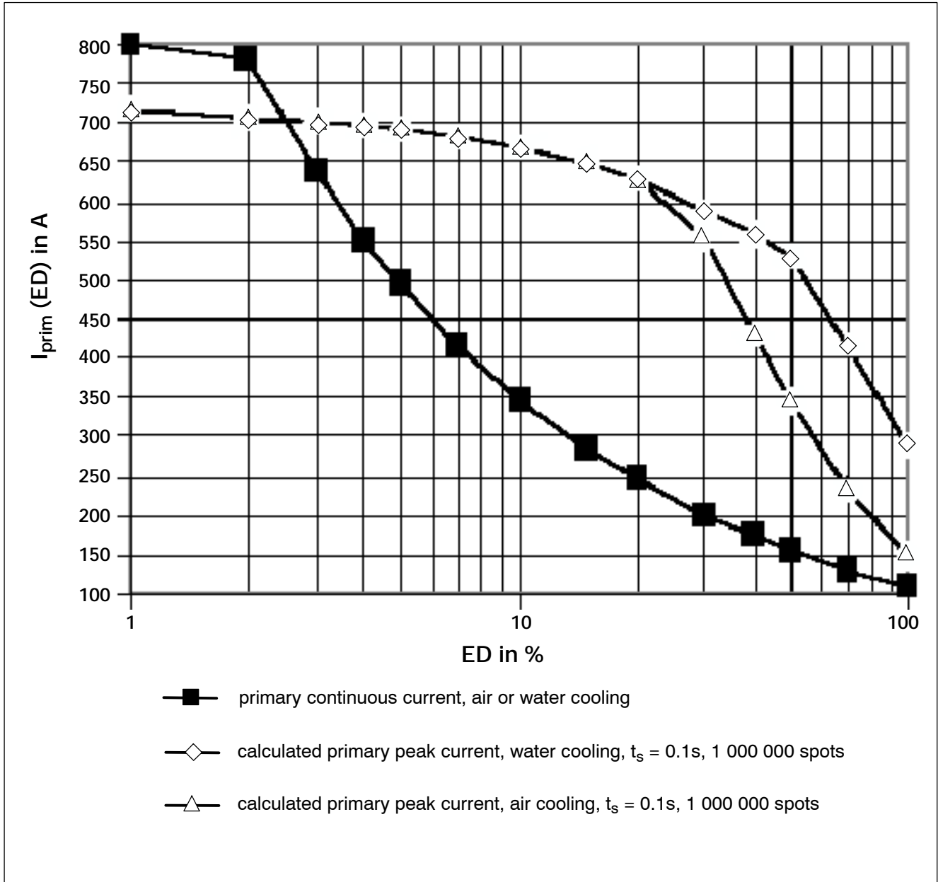
Load diagram, PSI 6300.XXX L2/W2
