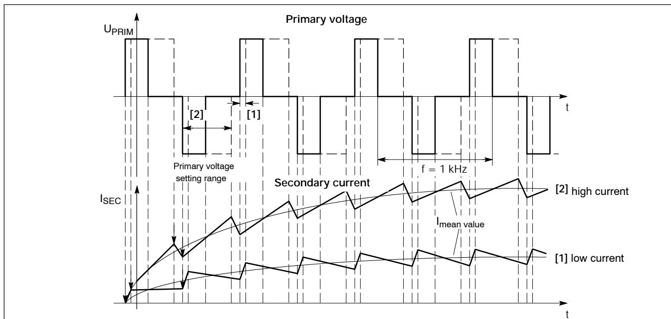
Primary and secondary voltages for medium-frequency welding
