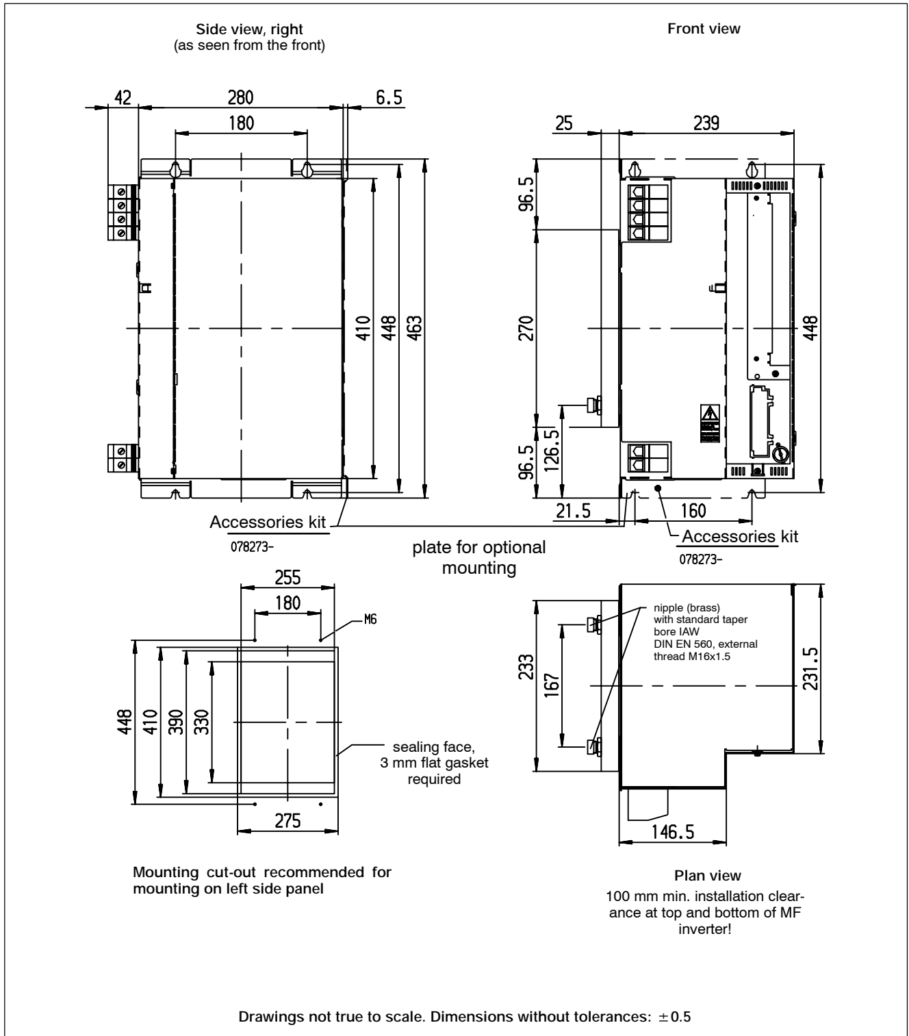
Dimensioned drawing, PSI 6100.XXX W1/W2
