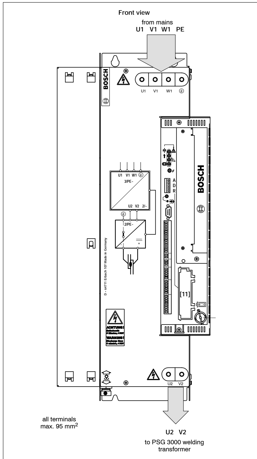
Electrical connection, PSI 6200.XXX W1/W2
