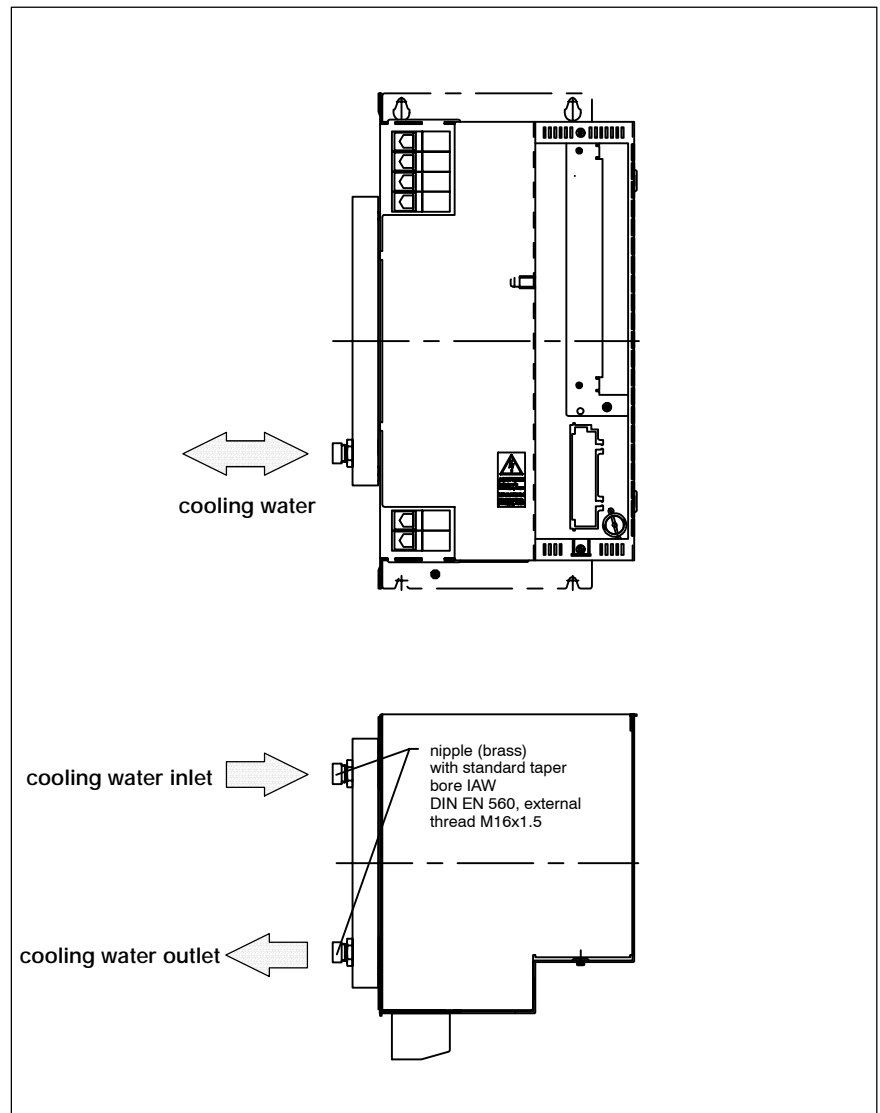
Cooling water connection, PSI 6300.XXX W1/W2
