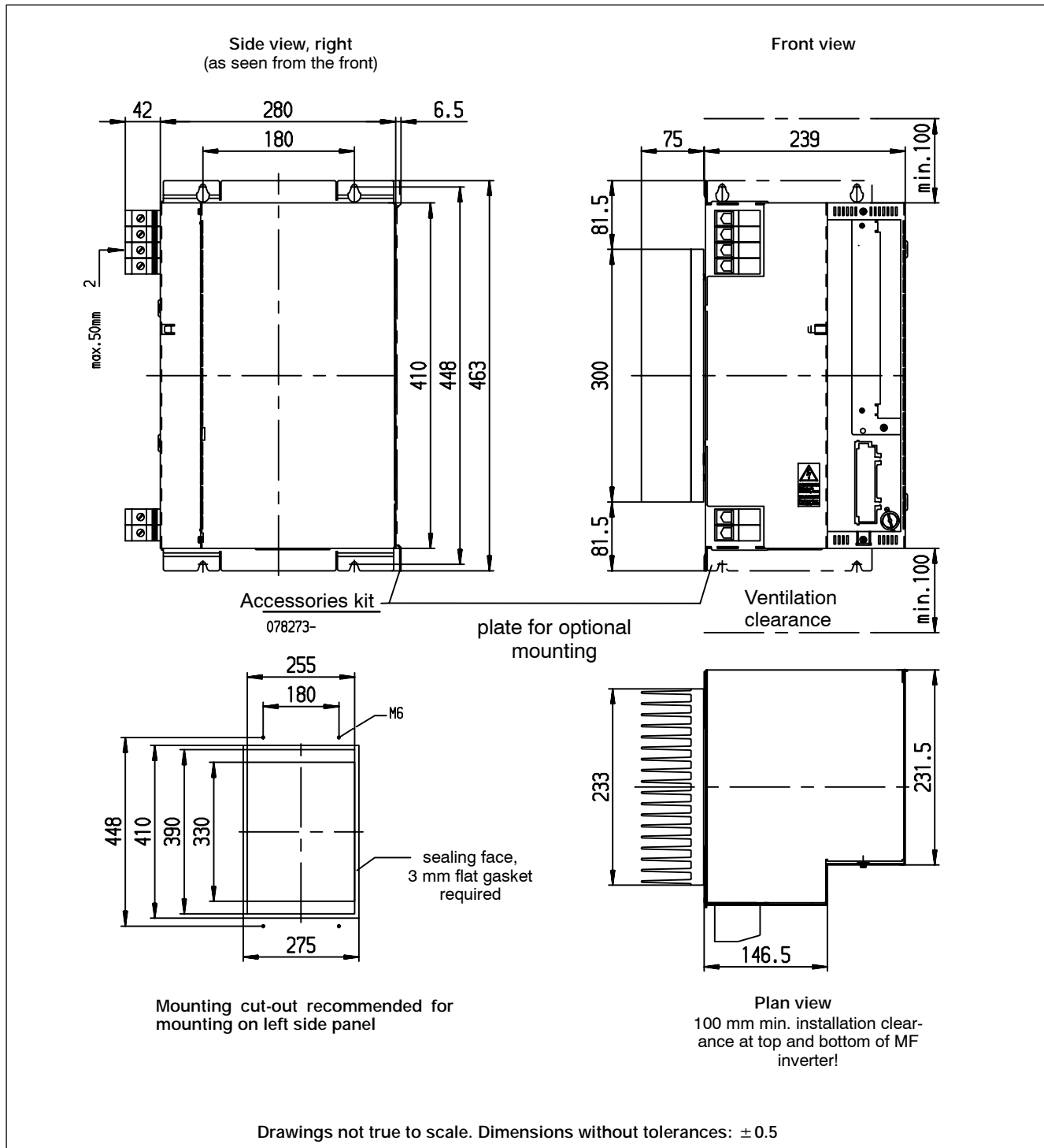
Dimensioned drawing, PSI 6300.XXX L1/L2
