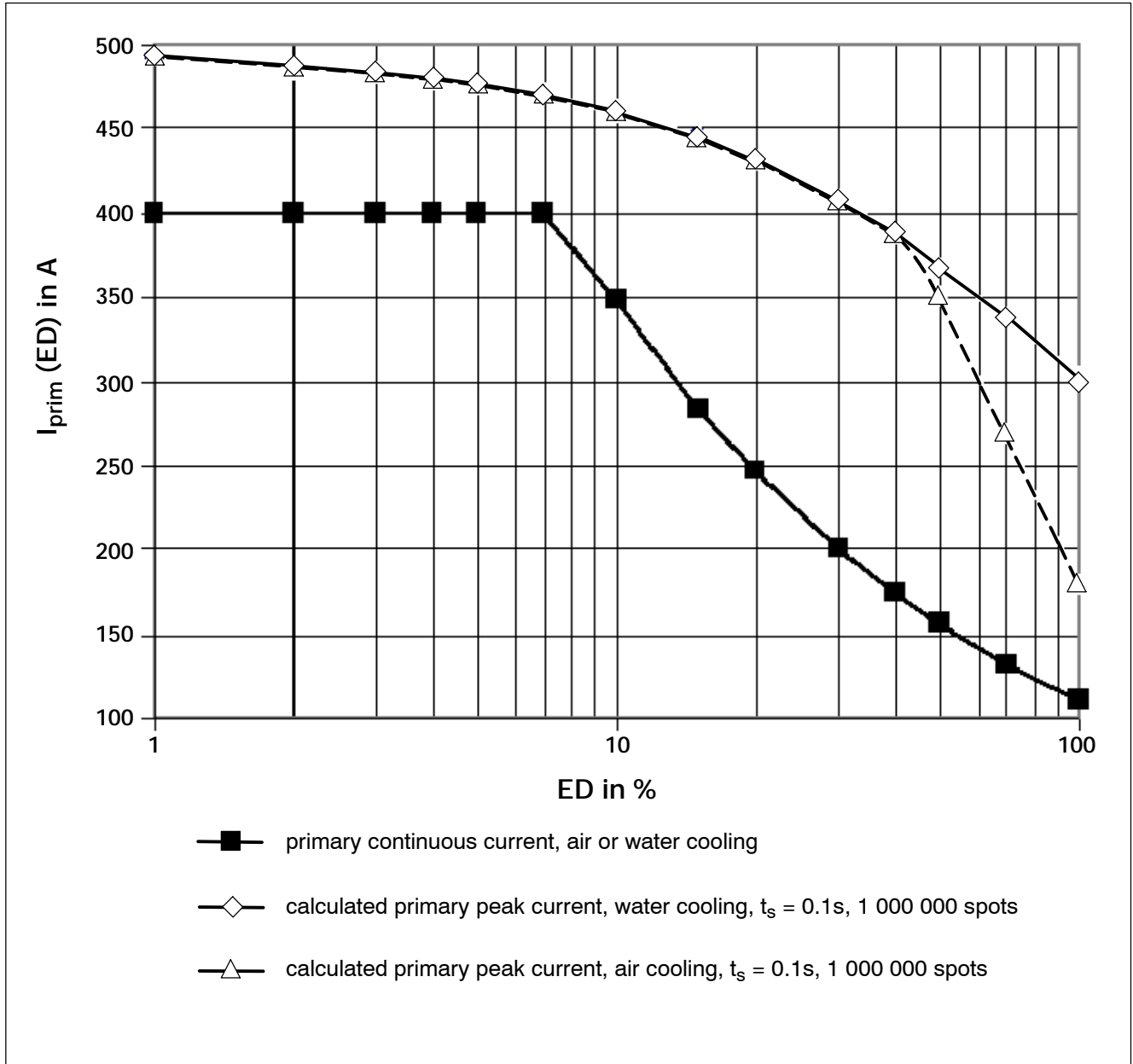
Load diagram, PSI 6100.XXX L1/W1
