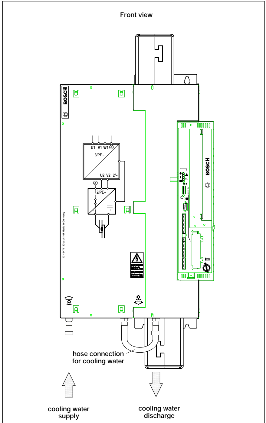
Cooling water connection, PSI 6500.XXX W1
