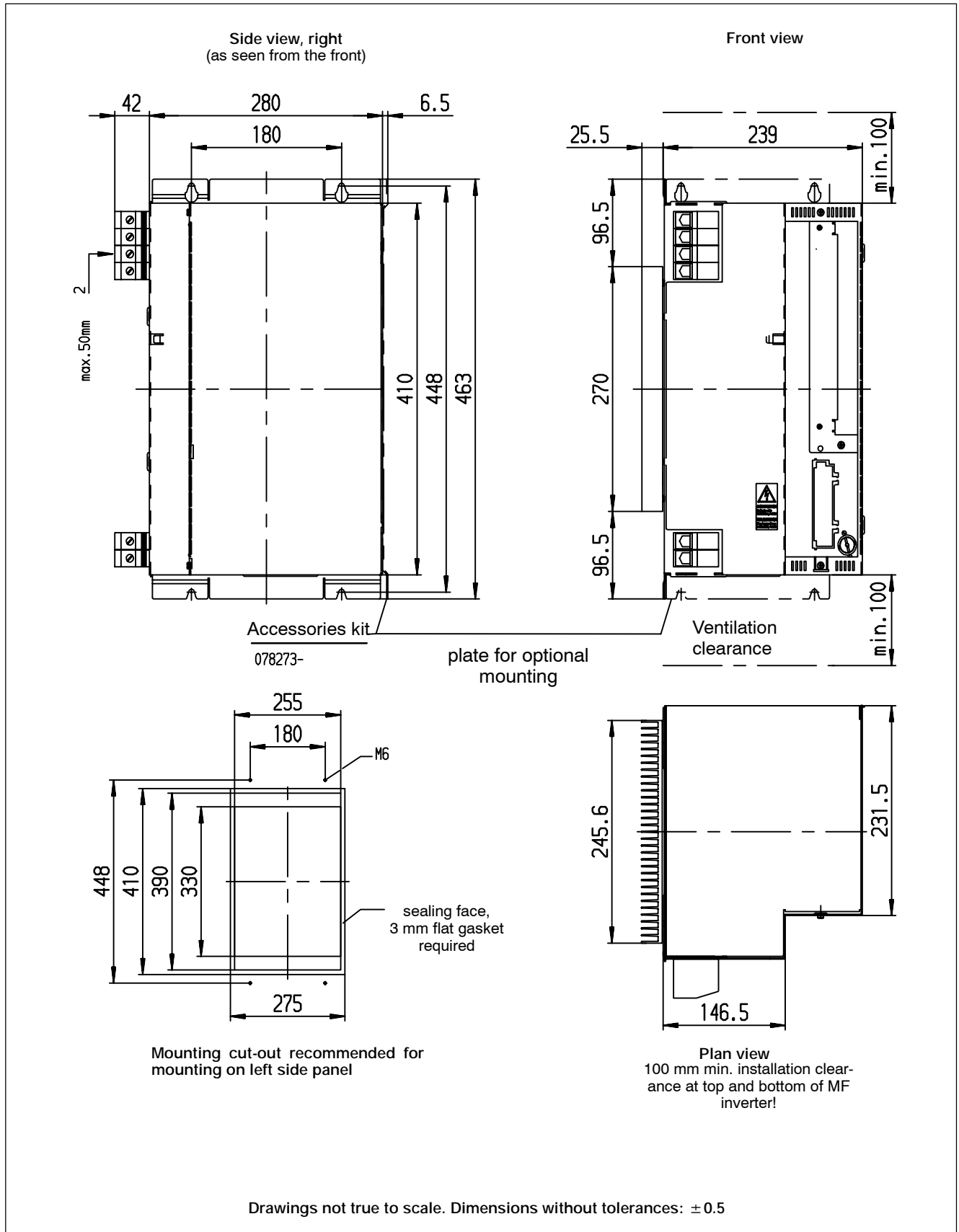
Dimensioned drawing, PSI 6025.XXX L1
