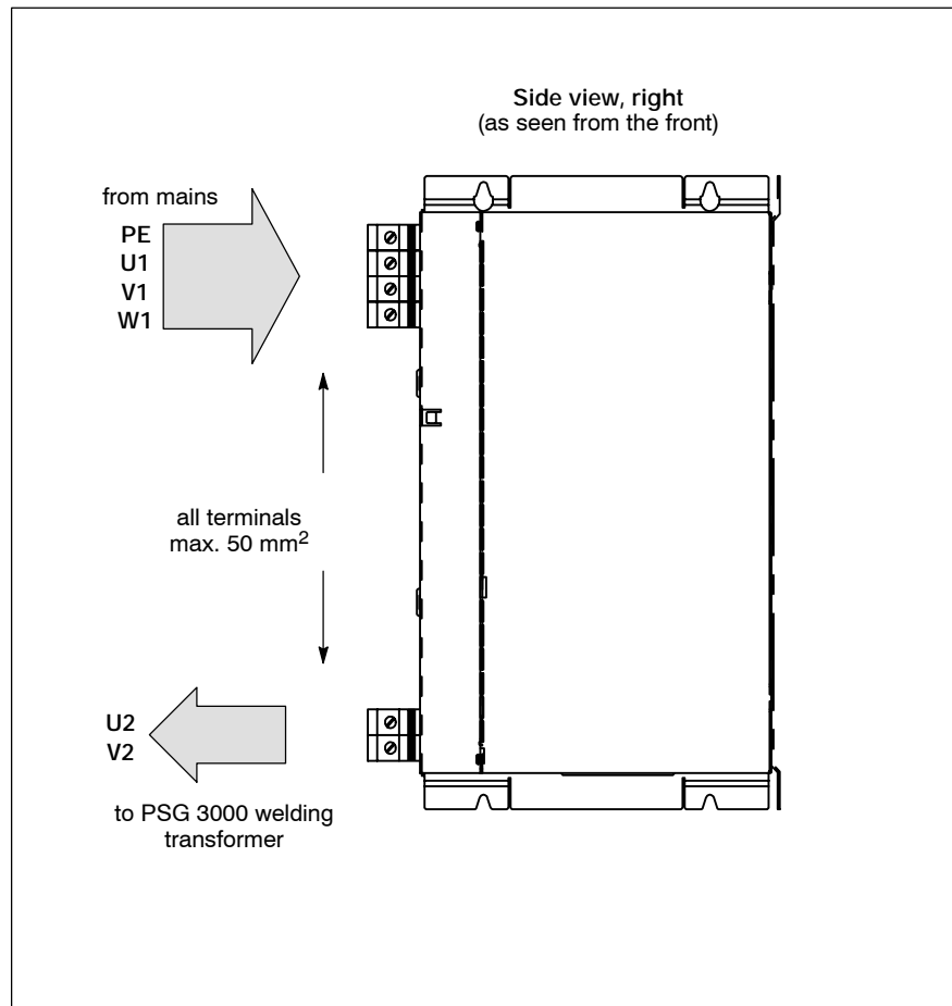
Electrical connection, PSI 6025.XXX L1
