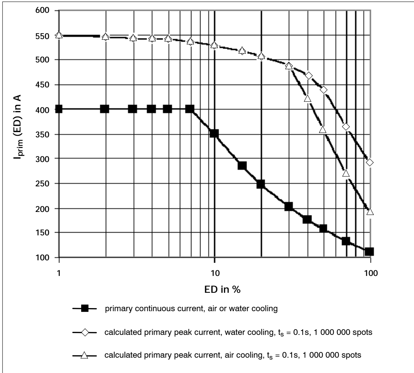
Load diagram, PSI 6100.XXX L2/W2
